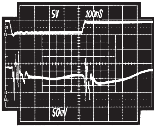
Figure 8B. Use of 0.1 \mu\text{F} Film Capacitors with no Bulk Capacitors
