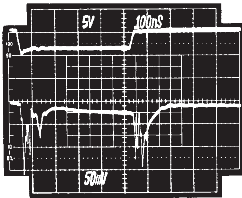
Figure 8C. Use of 0.15 \mu\text{F} Distributed Tantalums with no Bulk Capacitors
