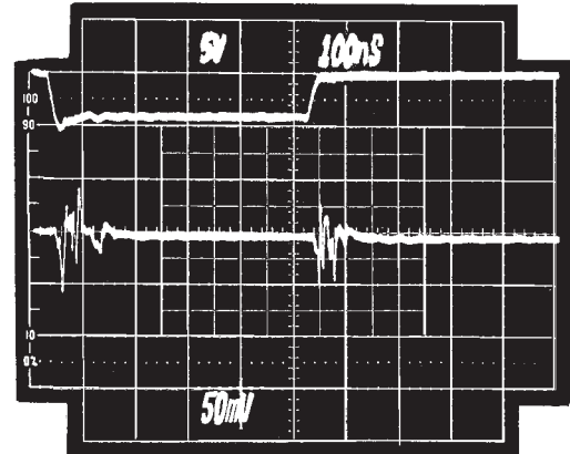
Figure 6A. Results of Increasing Value of Distributed MLCs to 1.0 \mu\text{F}
