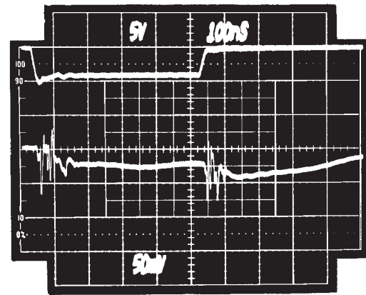
Figure 8E. Axial-lead MLCs Used for Decoupling with no Bulk Capacitors
