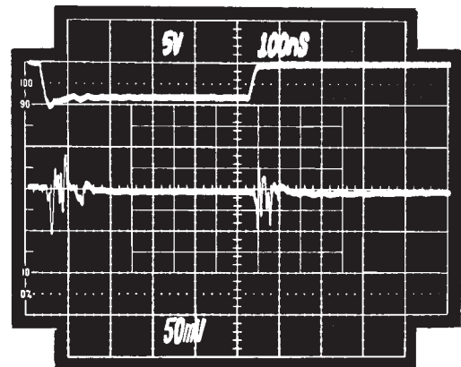
Figure 6B. Adding Bulk Capacitors to 1.0 \mu\text{F} Distributed MLCs has no Effect on Waveform
