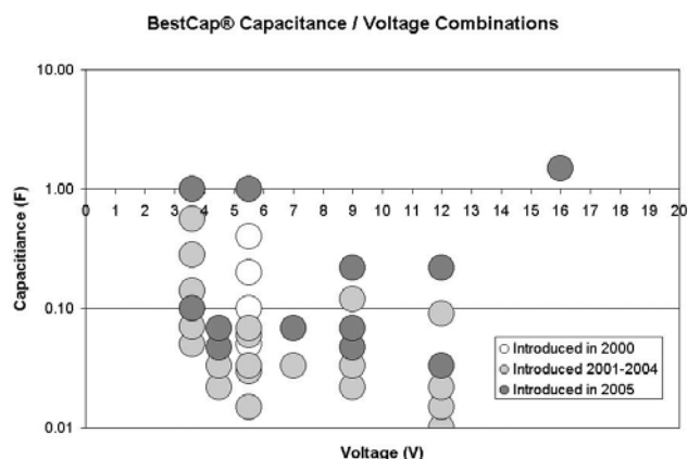
Figure 1: BestCap® Capacitance and Voltage Combinations Available.
