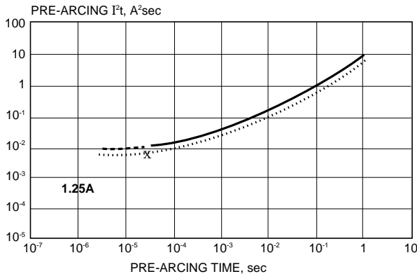
Fig. 4c. Choice of 1.25A fuse, example #4.
