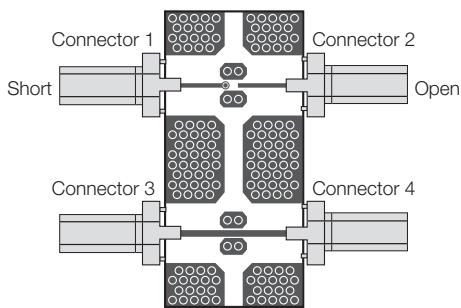
Measurement Jig
