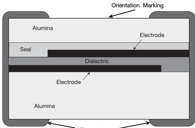
Figure 3. Accu-P® Capacitor Structure
