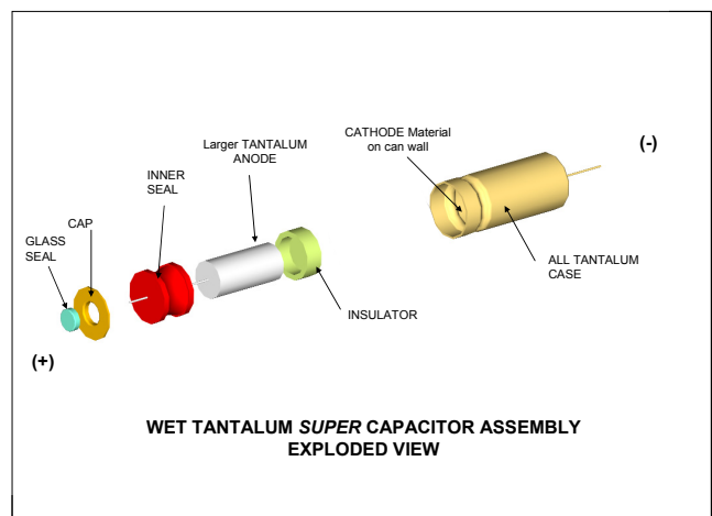
Fig. 1b – AVX TWA series wet tantalum construction
