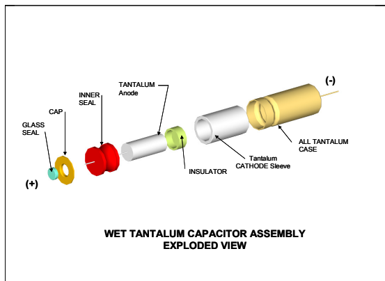
Fig. 1a – conventional wet tantalum construction
